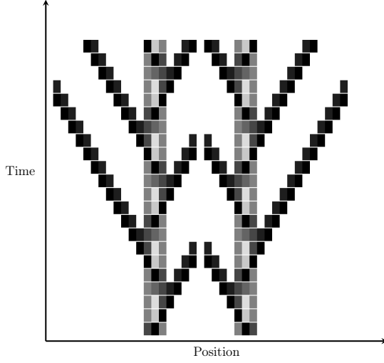
Figure 9: Two inward-facing initial states, with 9 cells inbetween
