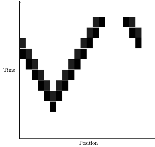
Figure 1: Evolution from a single excited cell with peridoic boundary condition
